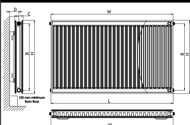
Type 21 - Technical Drawing
