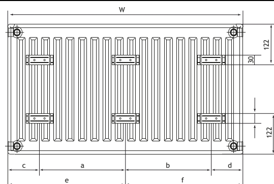
Bracket Positioning
