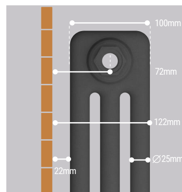
Pictured 41.0979 Matt Anthracite with 41.0360 feet
