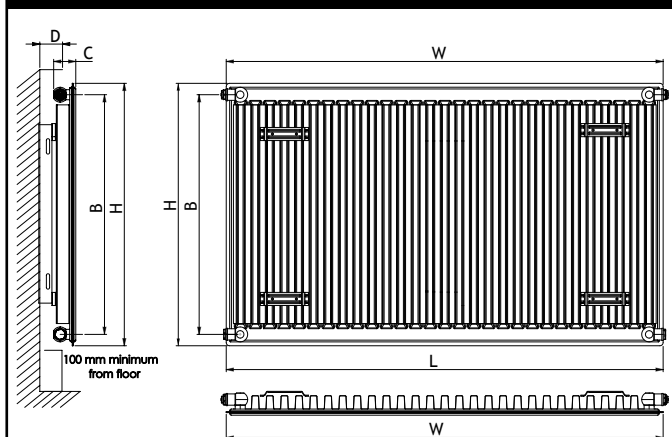
Type 11 - Technical Drawing
