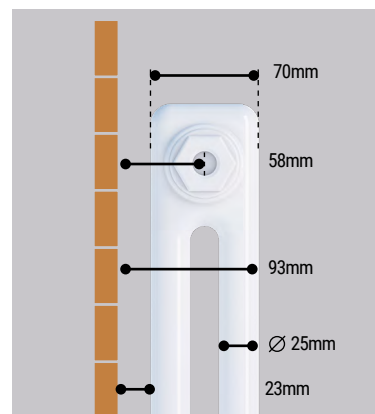
Pictured 81.0008 Gloss White with 81.0034 Feet and 8.541 Type H element
