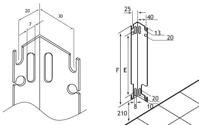
Wall Brackets
